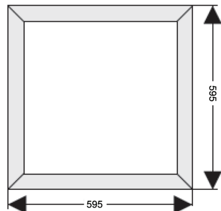
Micro-prismatic diffuser
